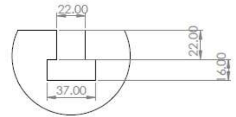
DETAIL A SCALE 1 : 2
