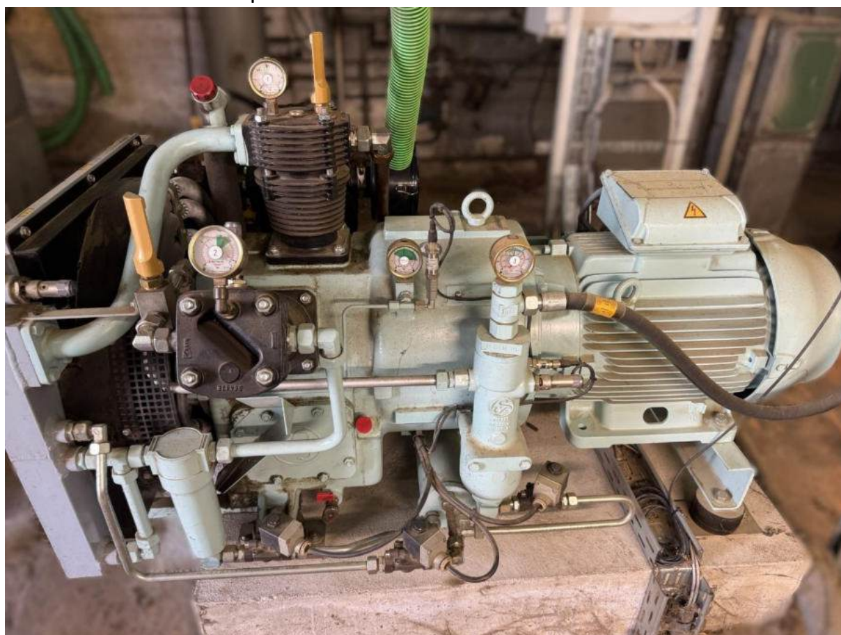
HD Compressor J.P. Sauer & Sohn WP 121L - 2016
