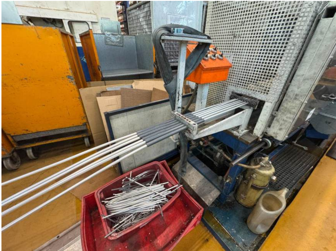
Pipe Fork Bending Machine 2 OAK TOOLS 6 & 10 mm
