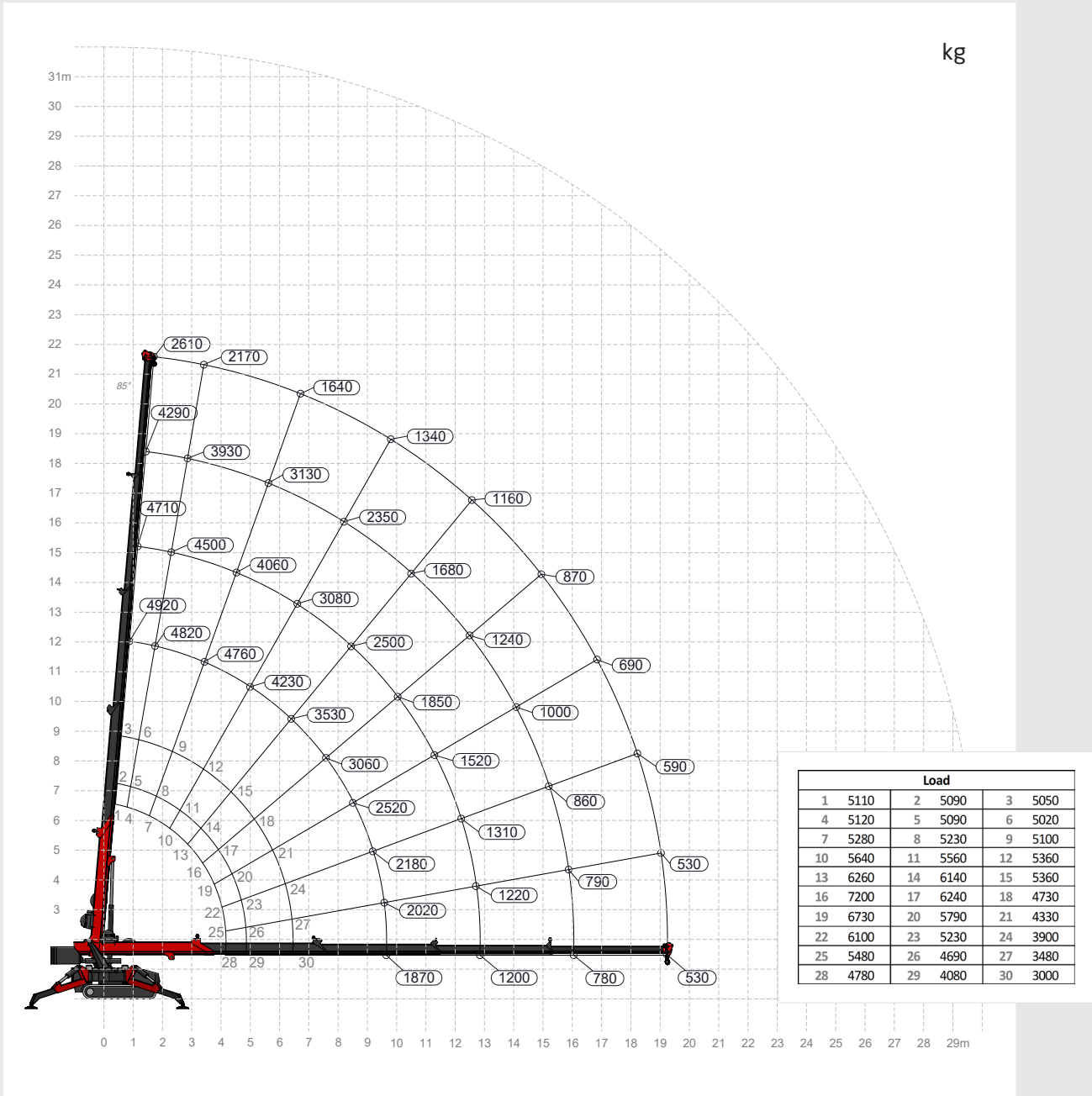
Main boom
