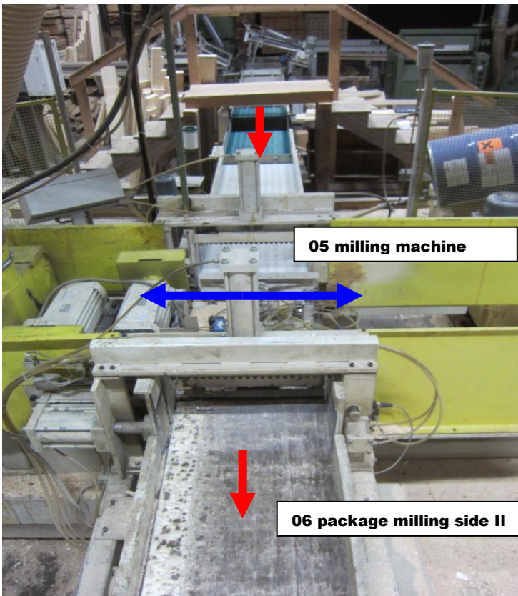
04 package milling side I
