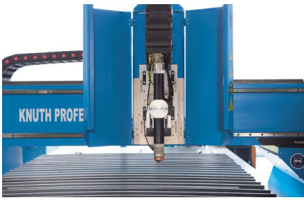
Quick-coupling for cutter head
