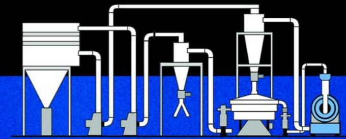
Pulverizer system with screening machine
