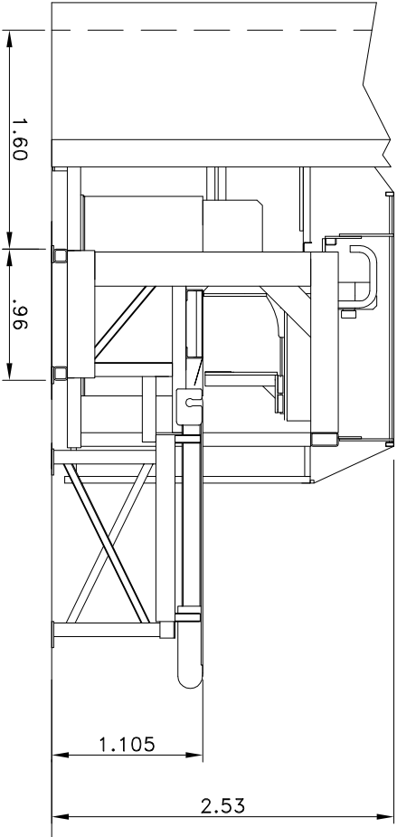
View X M 1:50
