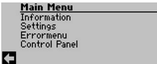
Figure 22: Main menu
