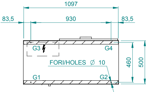
IMPRONTA A TERRA / FOOTPRINT
