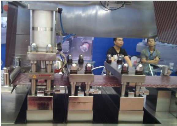
Heat-sealing, perforation and batch number embossing station
