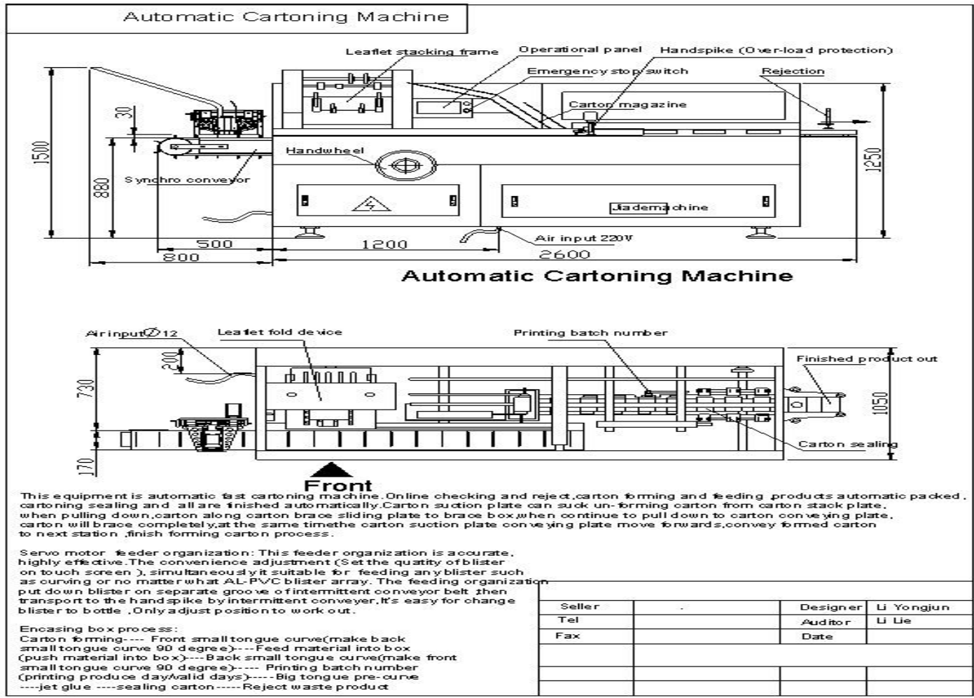
Working principle drawing
