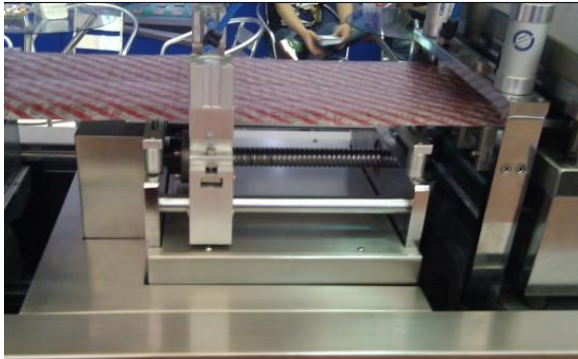
Heat-sealing, perforation and batch number embossing station
