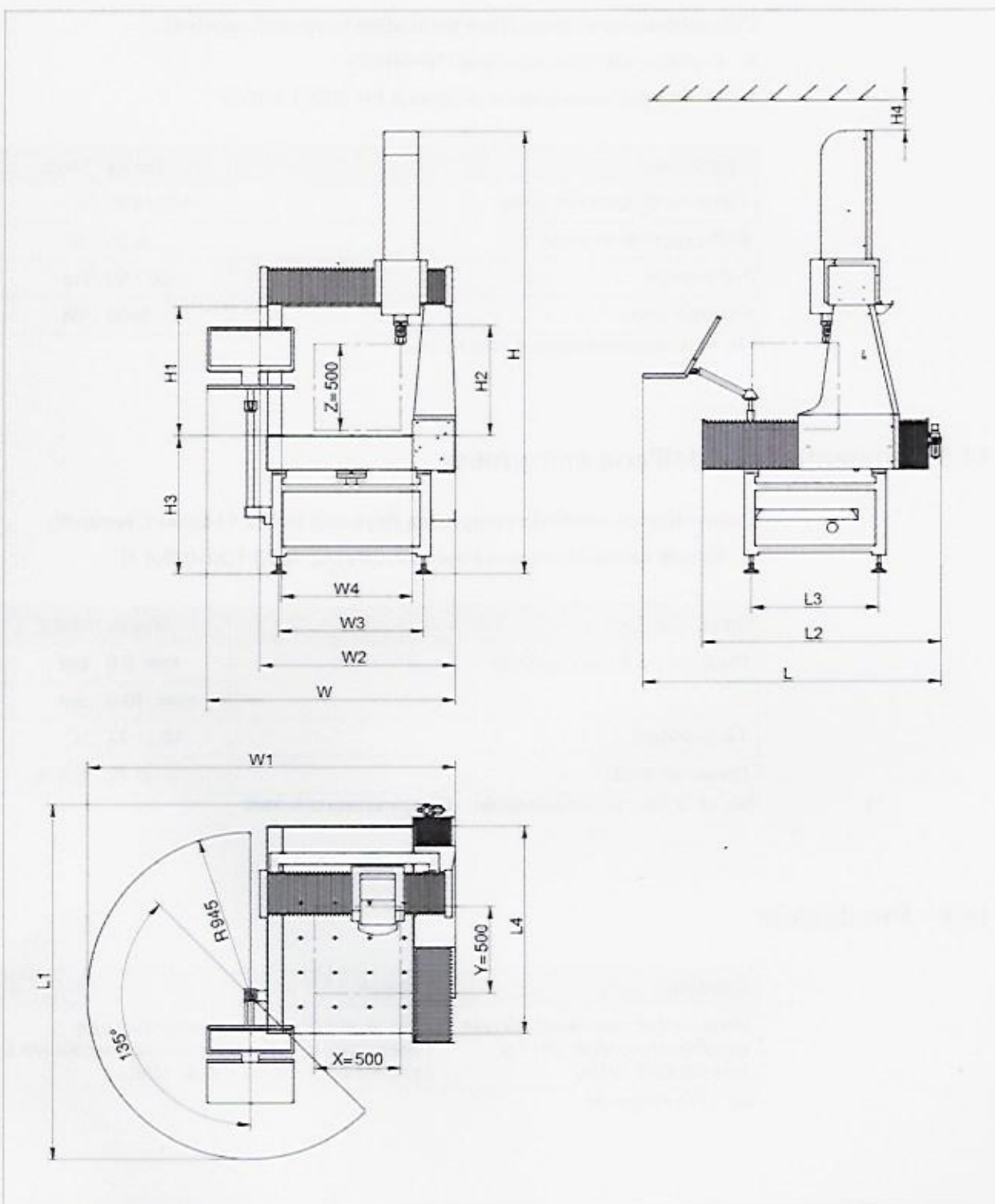
Fig. 14.54: Layout SF 55
