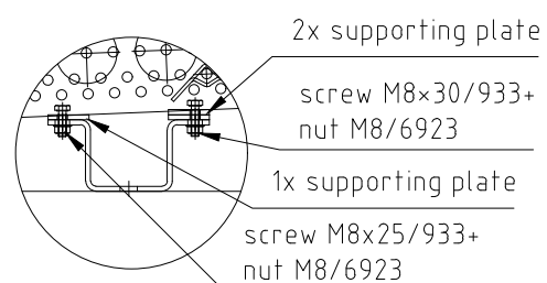
Detail "Stands UB-130 with supporting plate
