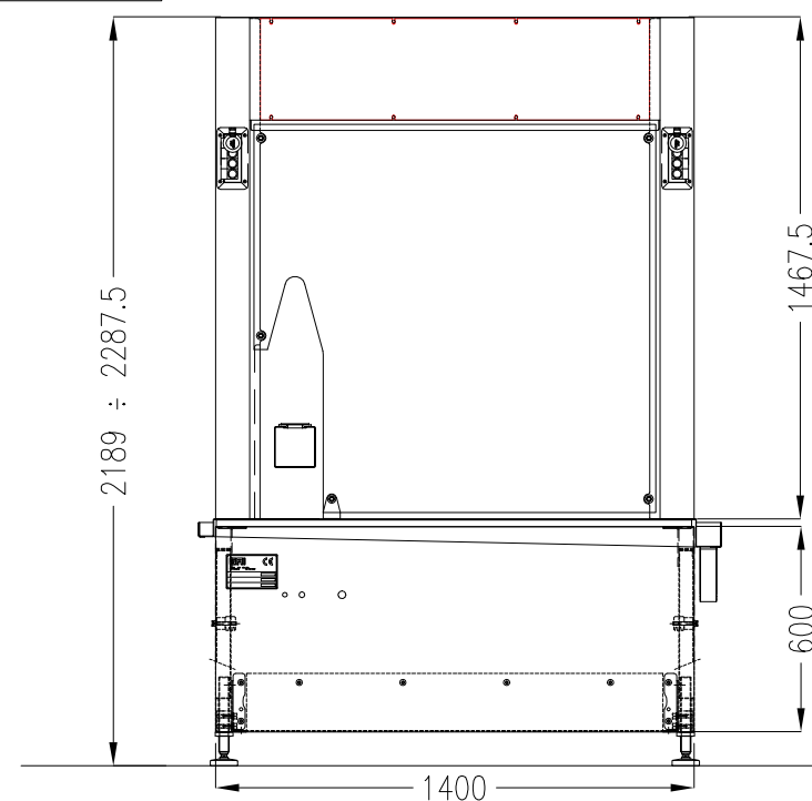
View "A"
