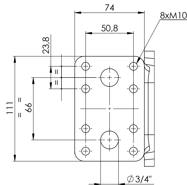
Hydraulic motor flange
