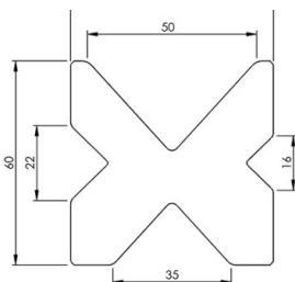
Machine is standard delivered with an European type bottom tool 4V
