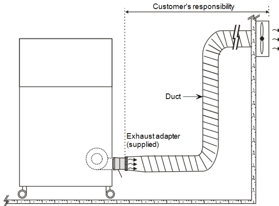
Figure 5 Printer exhaust system
