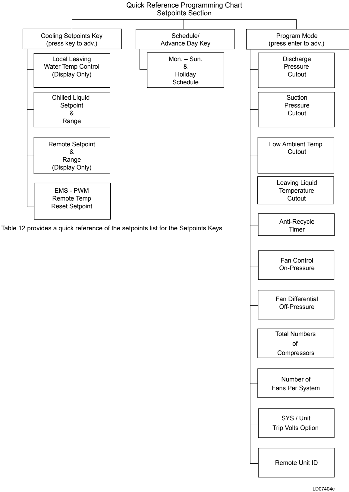
FIGURE 20 - SETPOINTS QUICK REFERENCE LIST
