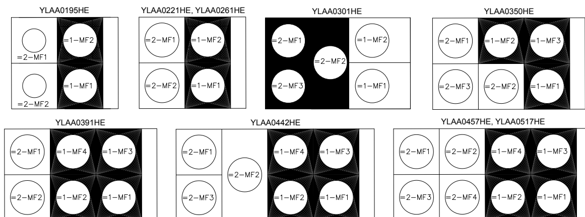
FIGURE 25 - CONDENSER FAN LOCATIONS
