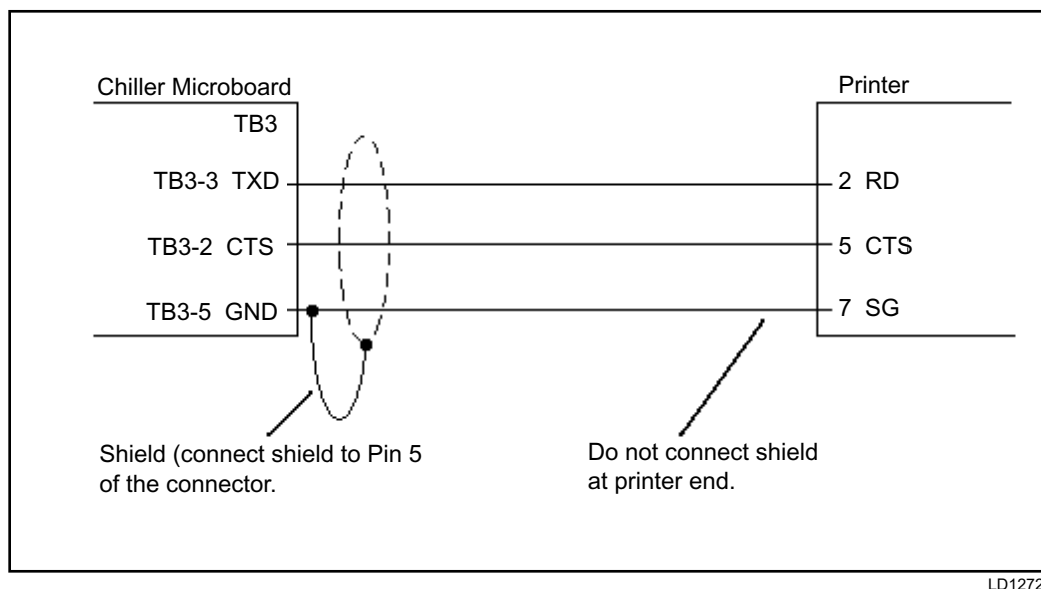
FIGURE 28 - PRINTER TO MICROBOARD ELECTRICAL CONNECTIONS
