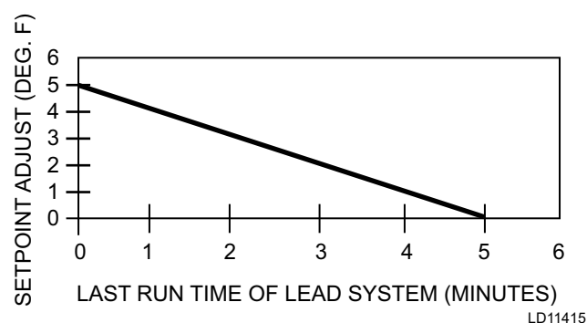
FIGURE 24 - SETPOINT ADJUST
