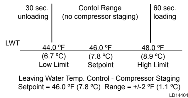
FIGURE 23 - LEAVING WATER TEMPERATURE CONTROL EXAMPLE
