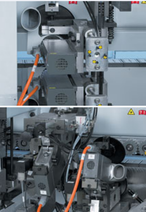
Trimming unit Trimming unit with DFC tool technology for optimum extraction. Equipped with servo axis to adjust the unit automatically to edge thickness and profile.
