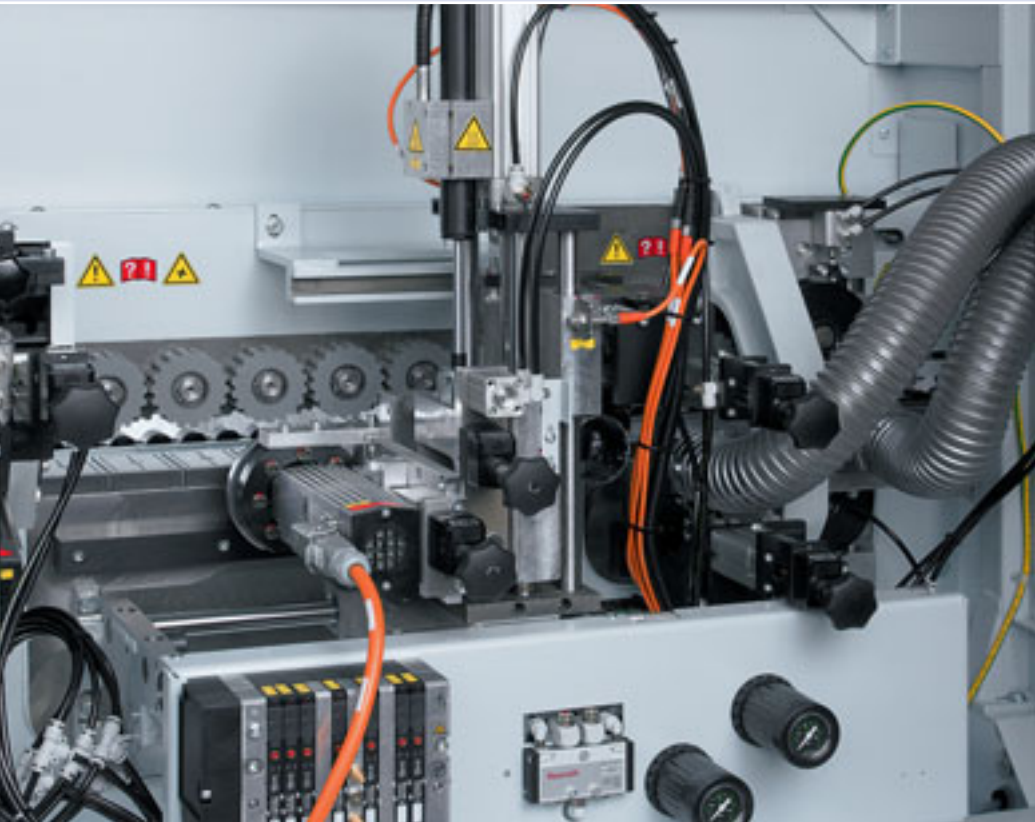
Corner rounding unit FF 10 (Highflex 1430) Optimum corner rounding without adjustment or set-up, resulting from the coupled DIA tool and tracer roller. Workpiece thickness up to 60 mm.
