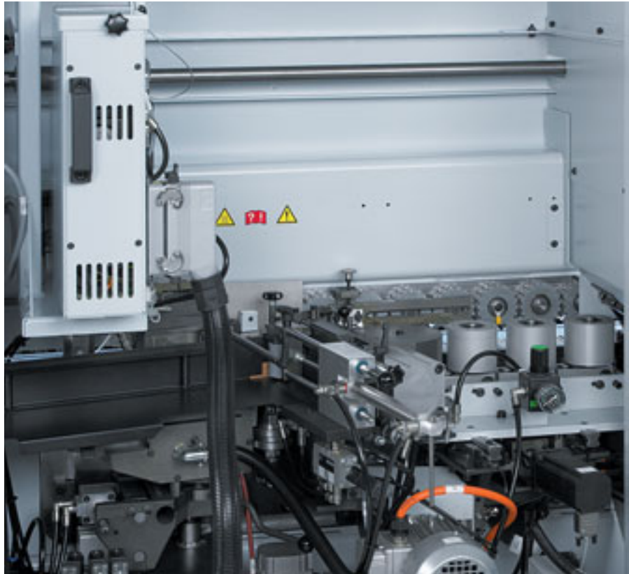
Magazine + pre-melter (optional) Coil and automatic strip magazine with optical monitoring for reliable material supply, high availability and perfect glue quality via the Quickmelt gluing unit.
