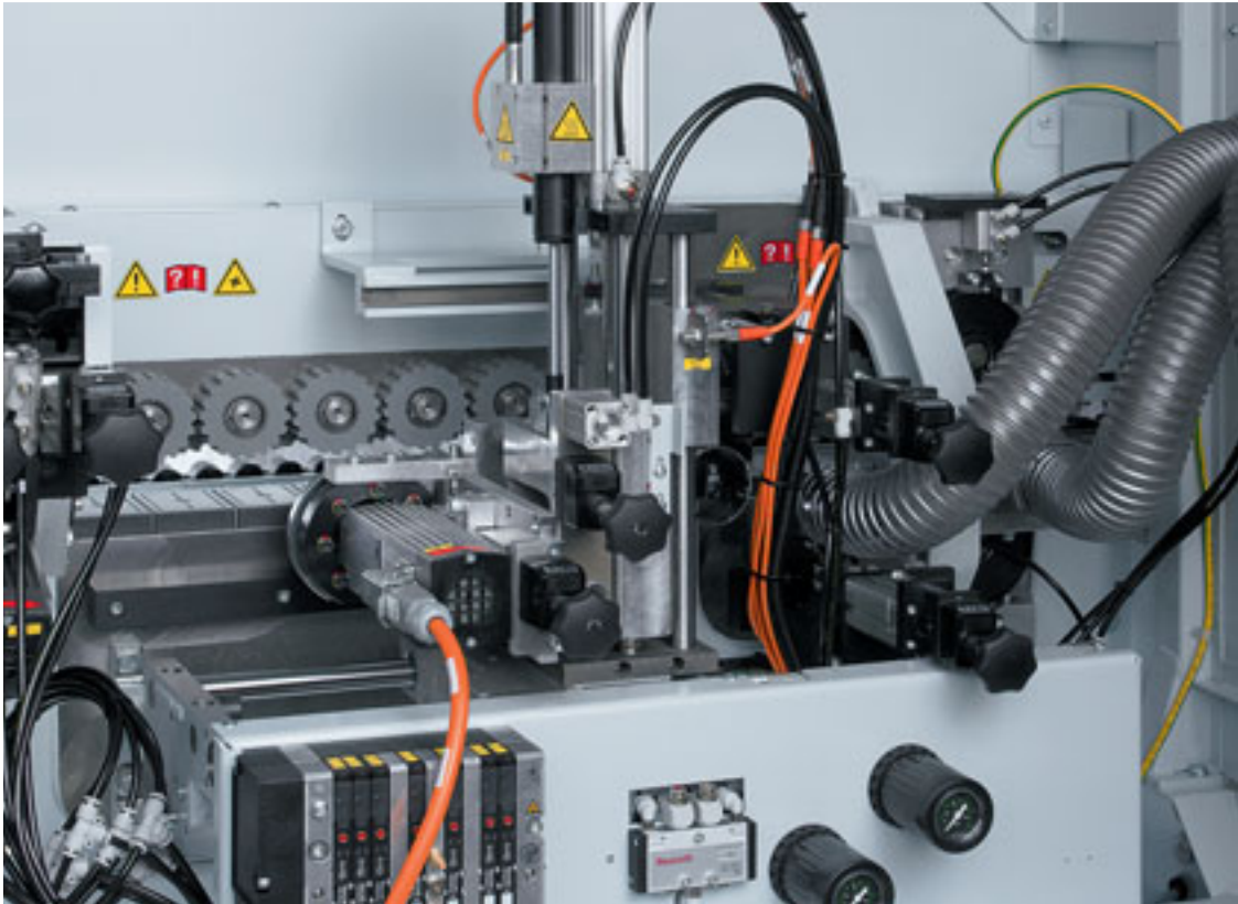
Corner rounding unit FF 10 Optimum corner rounding without adjustment or set-up, resulting from the coupled diamond tool and tracer roller. Workpiece thickness up to 40 mm. Workpiece thickness 60 mm - Highflex 1230.
