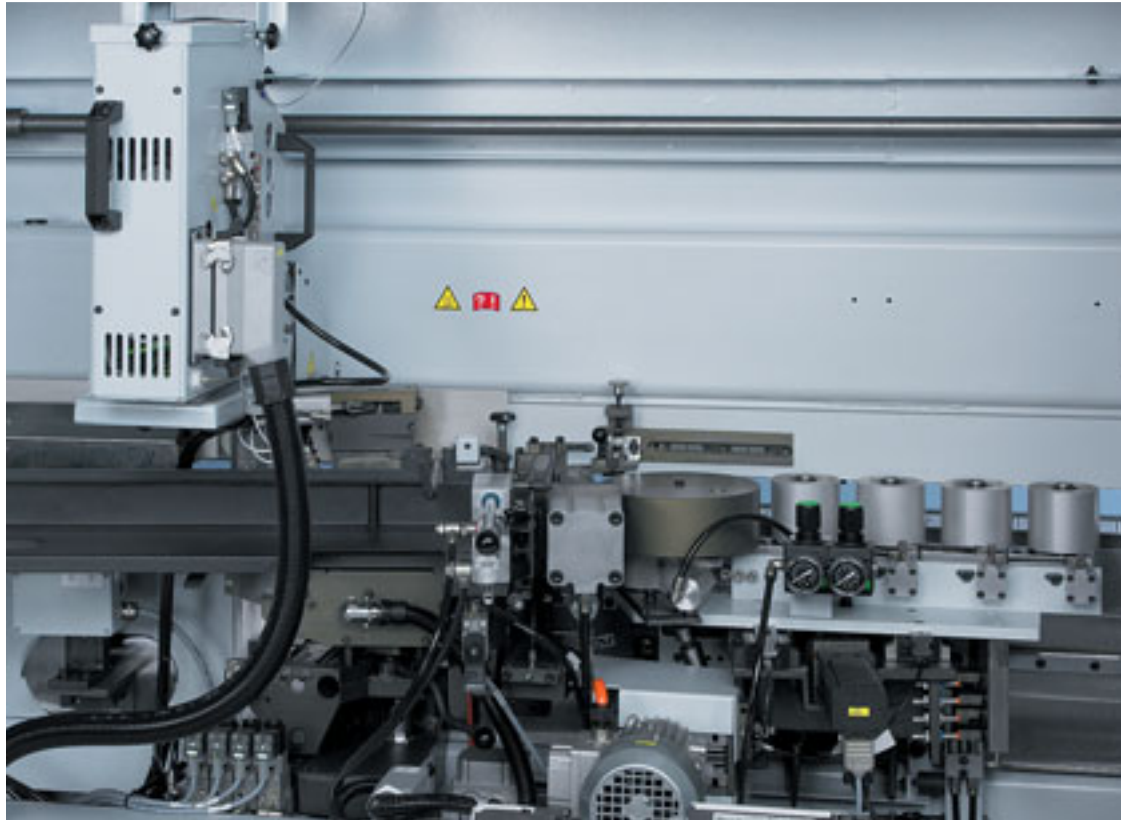
Magazine + pre-melter (optional) Coil and automatic strip magazine with optical monitoring for reliable material supply, high availability and perfect glue quality via the Quickmelt gluing unit.
