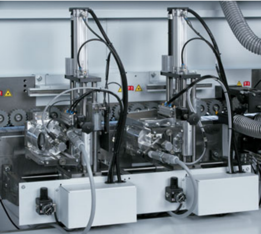
Multifunctional trimming unit MF 50 Trimming of the edge overhang on top and bottom side as well as contour trimming on the front and rear edges. Equipped with an automatic adjustment to switch between thick and thin edges. Workpiece thickness up to 60 mm.
