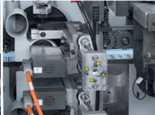
Rough trimming unit For rough trimming of all common edge banding materials.
