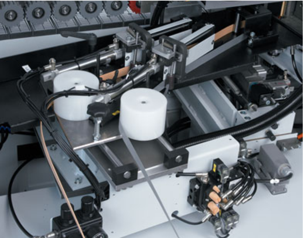
Automatic 2-coil magazine
