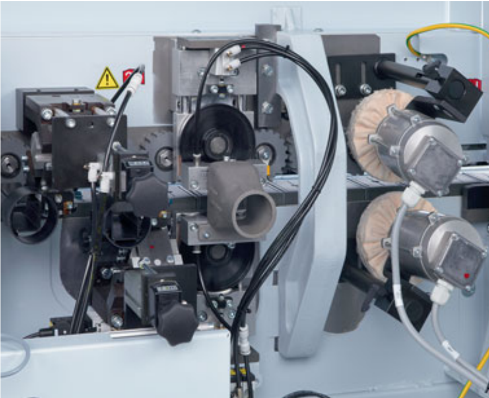
Profile scraping unit To smooth radii or chamfers (Pneumatic adjustment optional).
