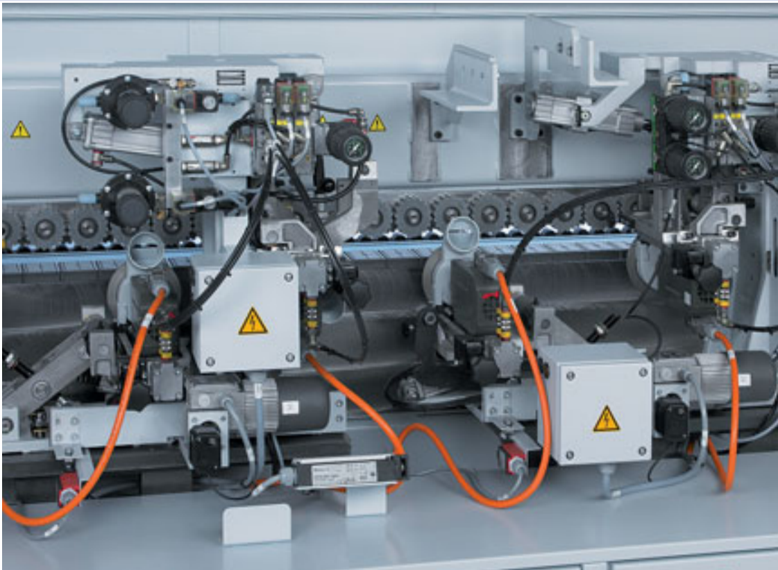
Corner rounding unit FF12 (4 motors) For corner rounding of thick PVC edges, as well as postforming and softforming profiles at feed speeds of up to 20 m/min. Equipped with servo motor adjustment for different edge thicknesses. Workpiece thickness up to 60 mm.
