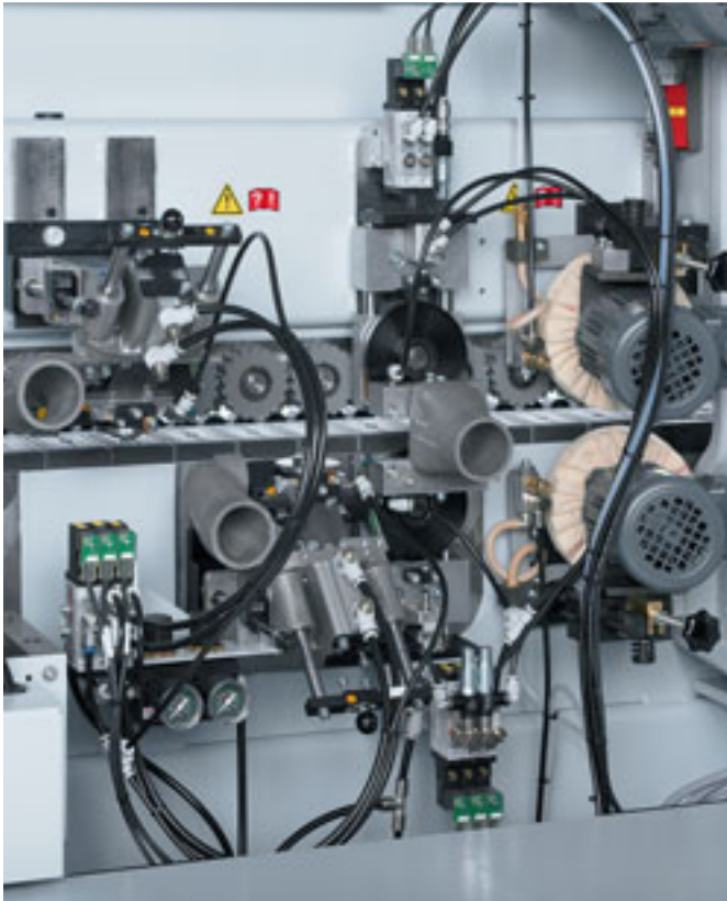
Profile scraping unit Unit to smooth radii or chamfers, equipped with quick change heads for fast profile change.
