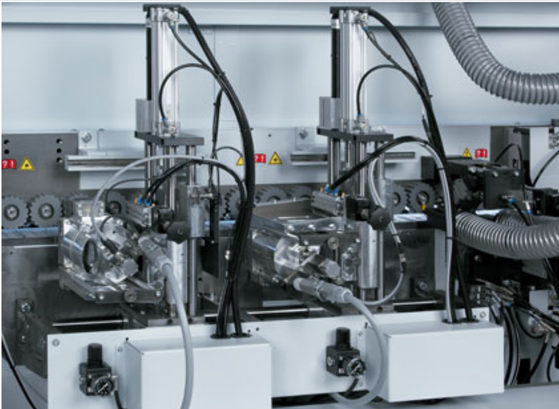
Multifunctional trimming unit MF 50 (Highflex 1440) Trimming of the edge overhang on top and bottom side as well as contour trimming on the front and rear edges. Equipped with an automatic adjustment to switch between thick and thin edges. Workpiece thickness up to 60 mm.
