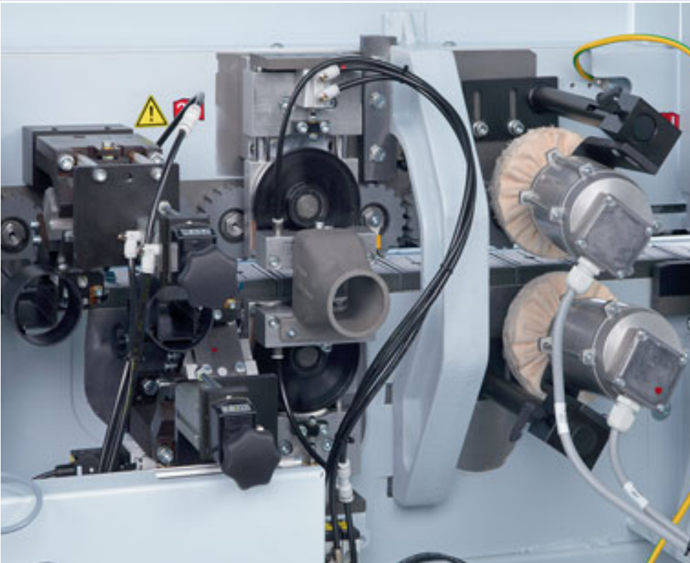
Glue joint scraping unit For the perfect finish.
