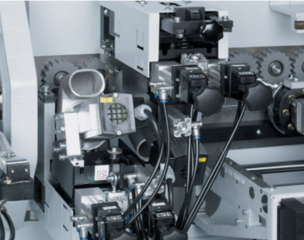
Trimming unit with pneumatic 3-point adjustment For even more effective production and much shorter changeover time.
