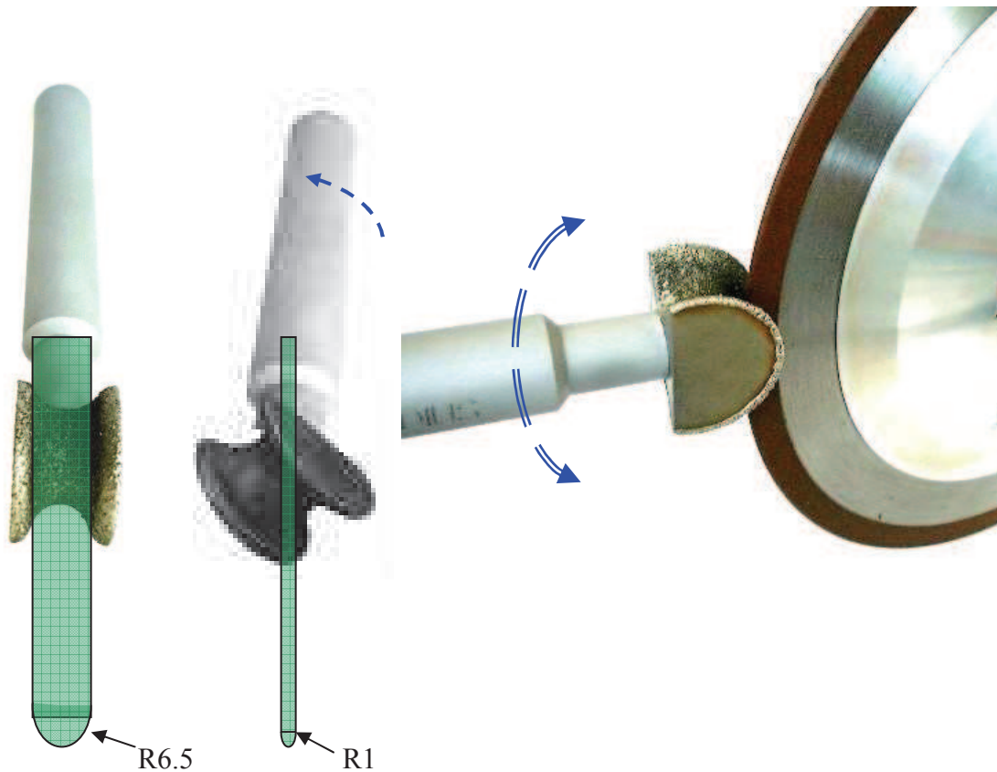
SETUP OF THE DRESSING DEVICE
