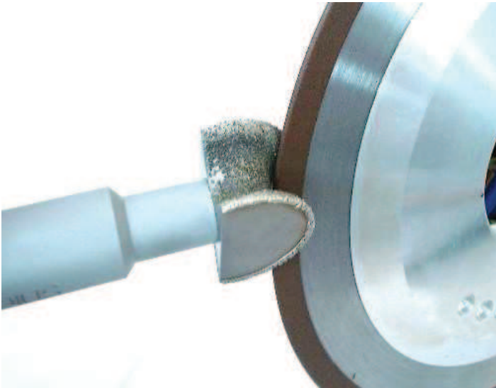
SETUP OF THE DRESSING DEVICE
