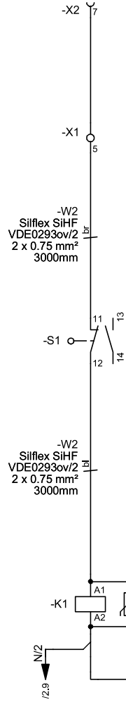
3RT1024-1AP00+VDR B 72220S271
