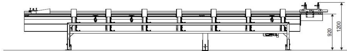
FRONT VIEW
