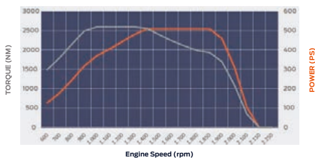
ECOTORQ GEN2 12.7 L EU6 510 PS
