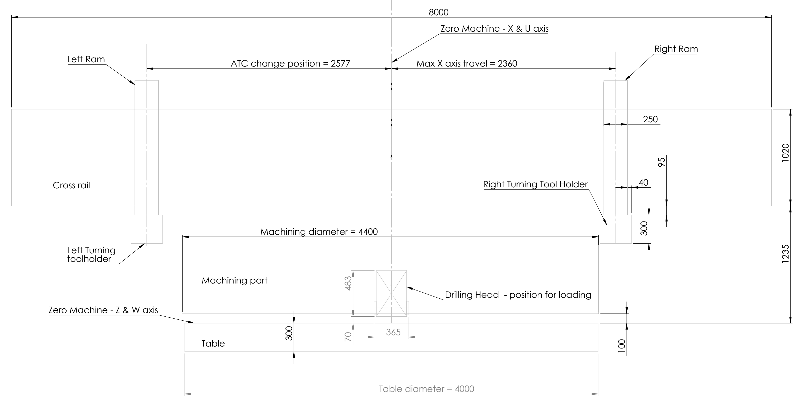
Work Space Diagram - SC 43 CNC 2SF
