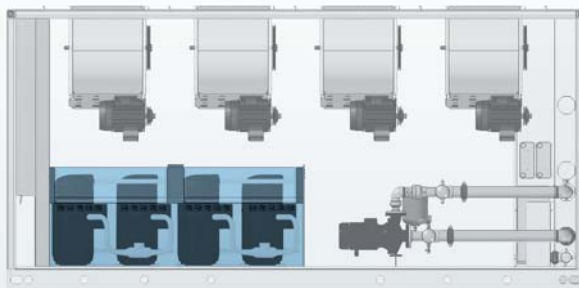
2 Pumps configuration (NECS-C 4 compressors)
